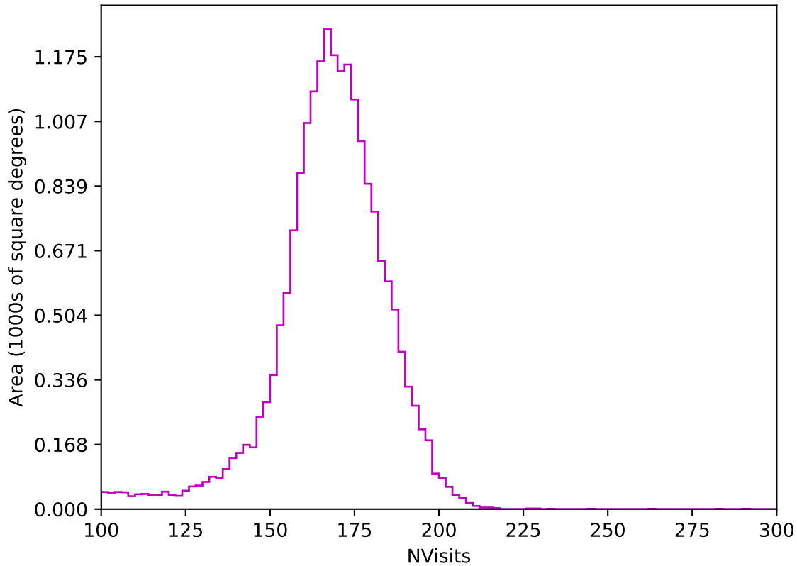
ddf_loaded_fl8_v3.4_10yrs All sky z band: NVisits
