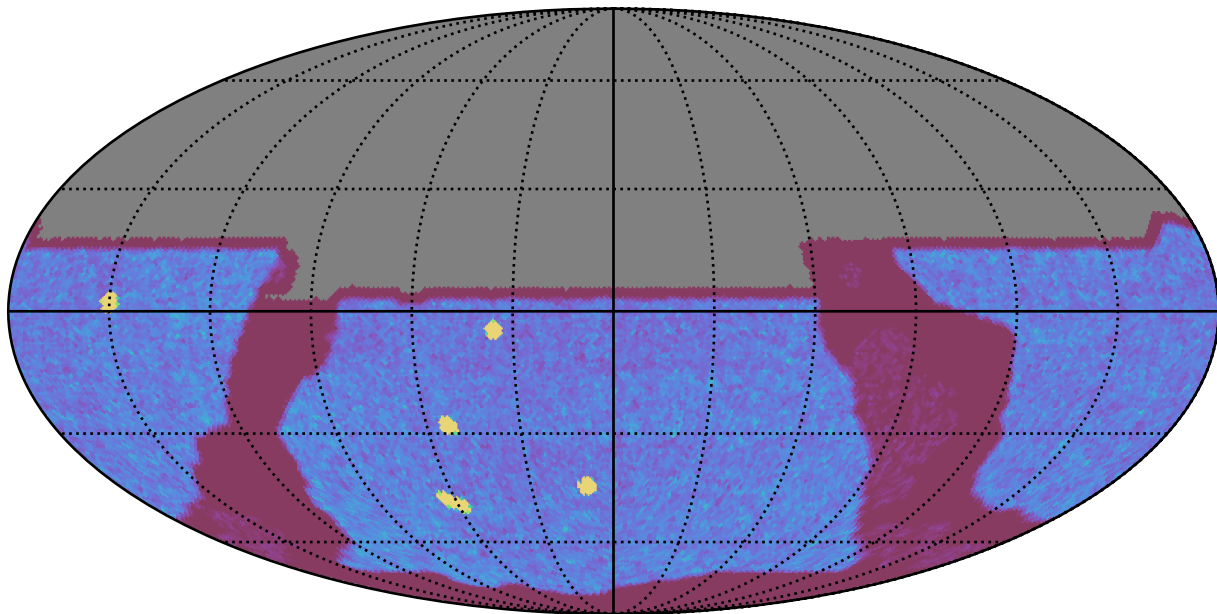
ddf_loaded_fl8_v3.4_10yrs All sky y band: NVisits
