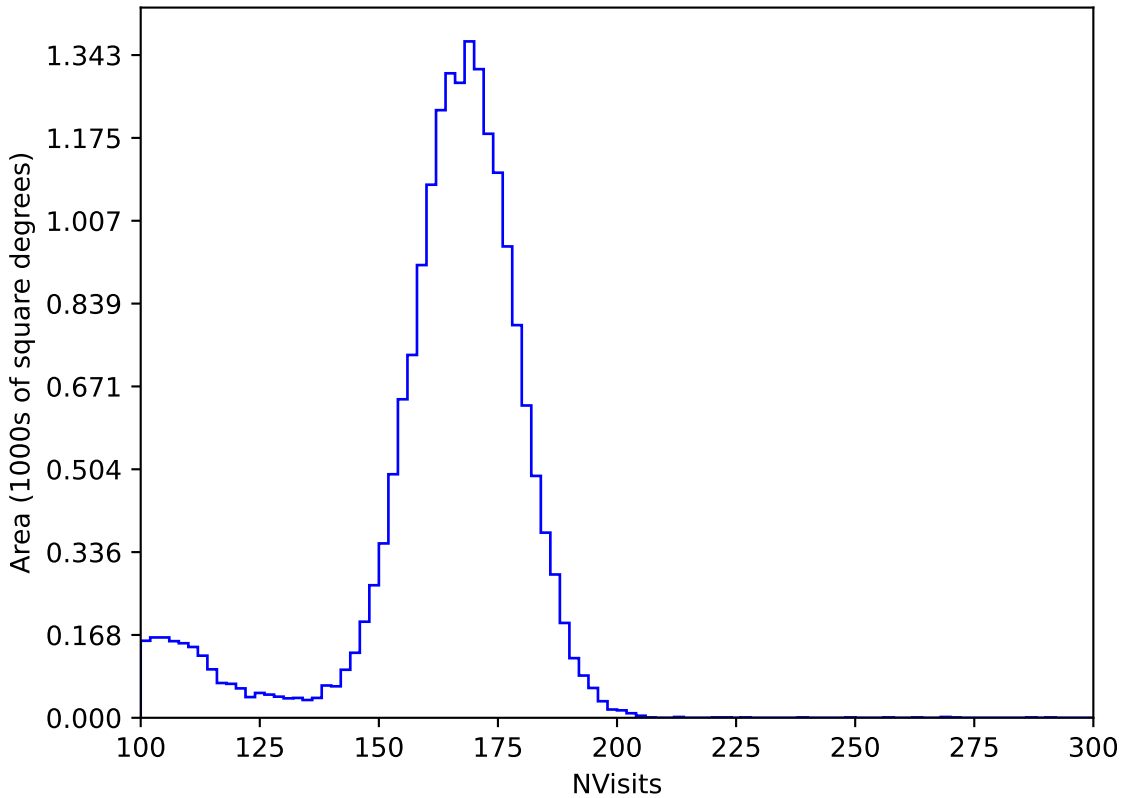
ddf_loaded_fl8_v3.4_10yrs All sky y band: NVisits
