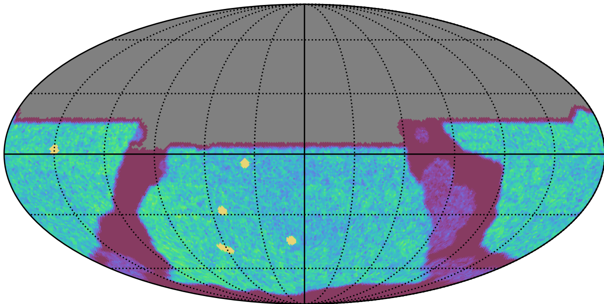
ddf_loaded_fl8_v3.4_10yrs All sky u band: NVisits
