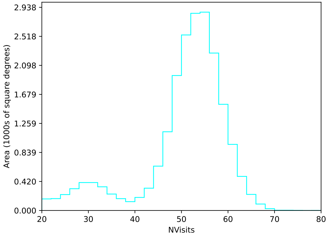
ddf_loaded_fl8_v3.4_10yrs All sky u band: NVisits
