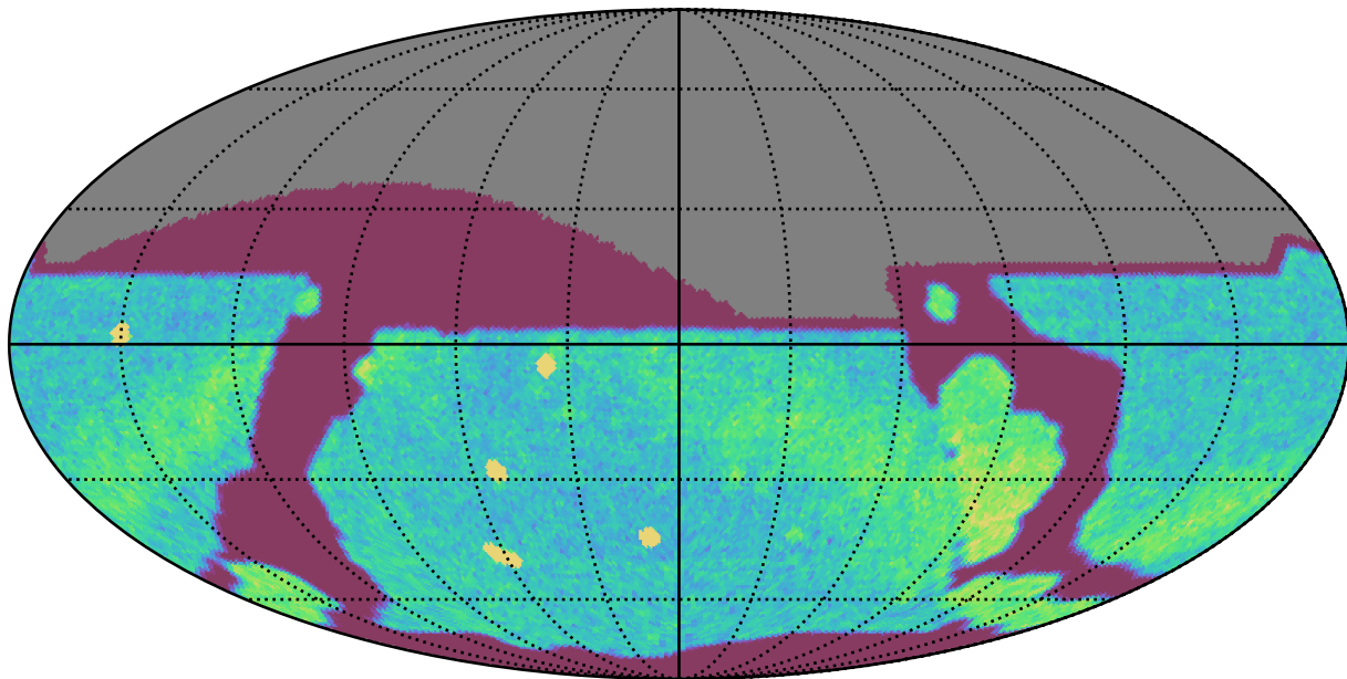
ddf_loaded_fl8_v3.4_10yrs All sky r band: NVisits
