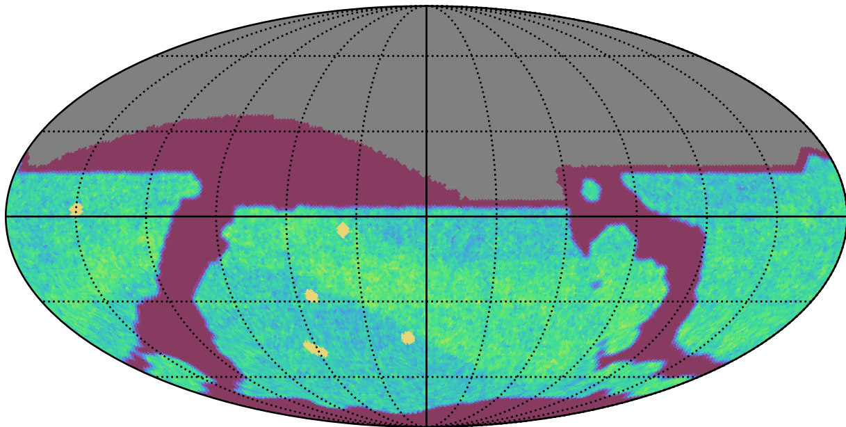
ddf_loaded_fl8_v3.4_10yrs All sky i band: NVisits
