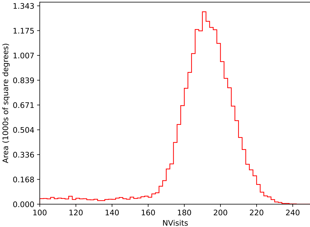
ddf_loaded_fl8_v3.4_10yrs All sky i band: NVisits
