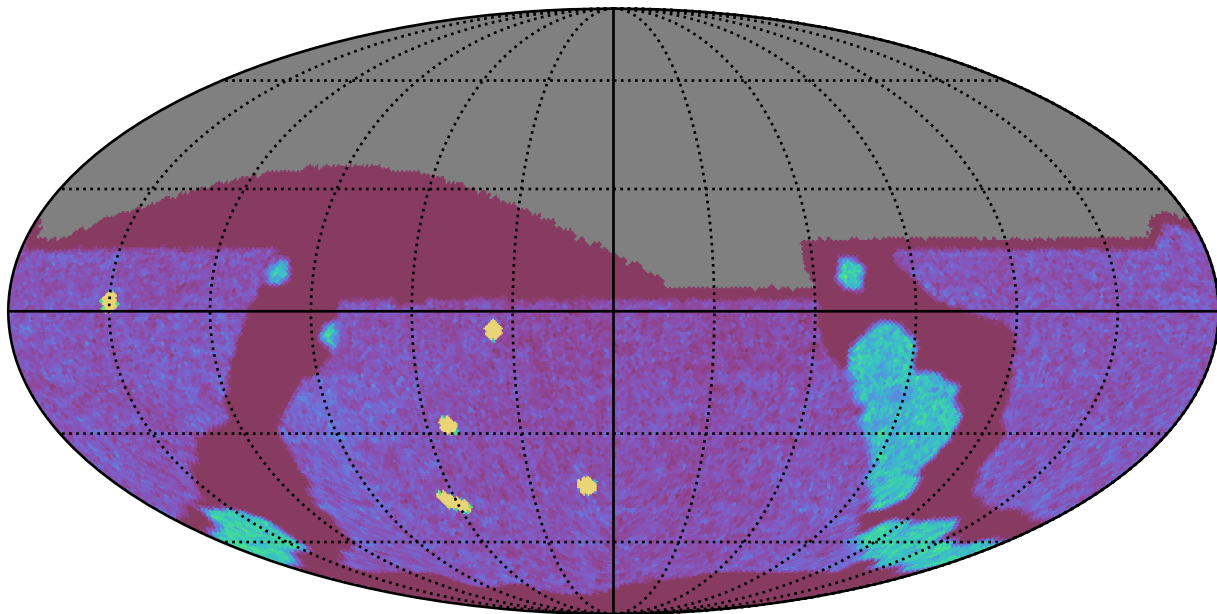
ddf_loaded_fl8_v3.4_10yrs All sky g band: NVisits
