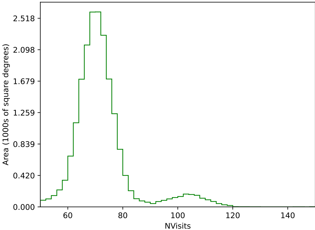
ddf_loaded_fl8_v3.4_10yrs All sky g band: NVisits
