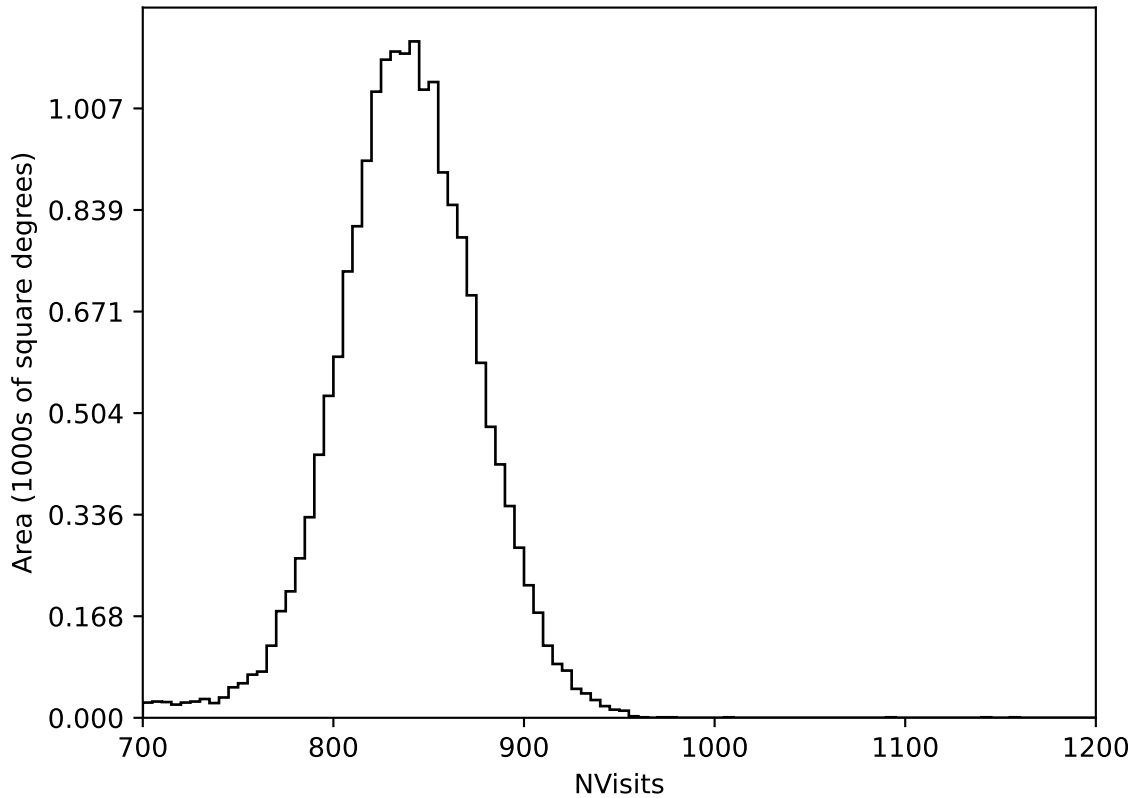
ddf_loaded_fl8_v3.4_10yrs All sky all bands: NVisits
