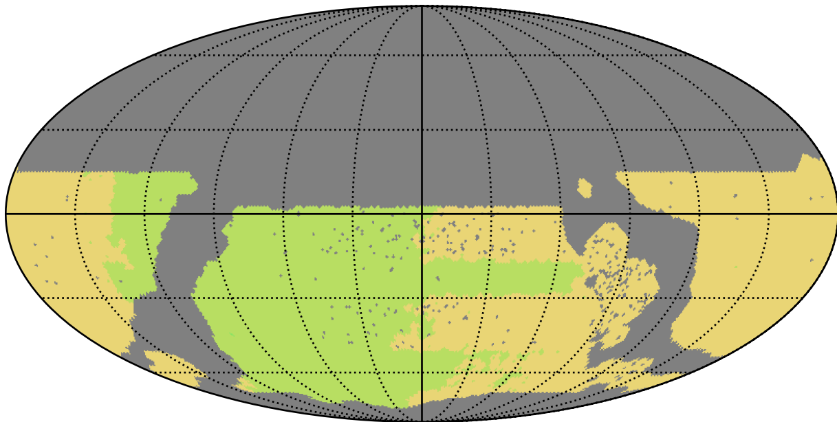
ddf_loaded_fl8_v3.4_10yrs WFD all bands: NSeasons
