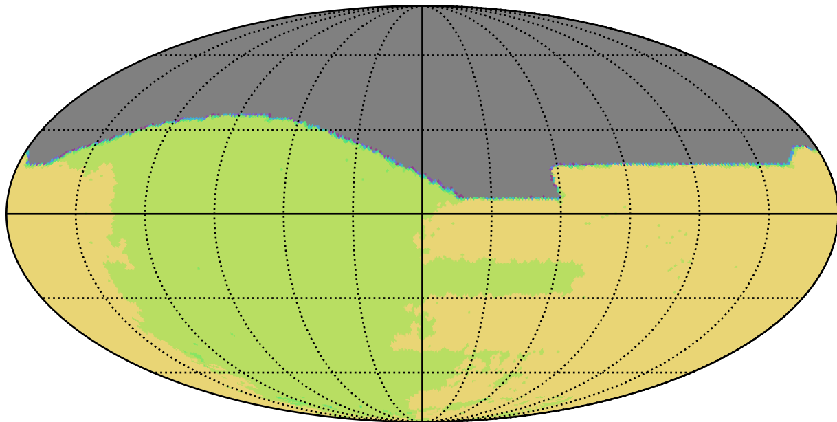
ddf_loaded_fl8_v3.4_10yrs All sky all bands: NSeasons
