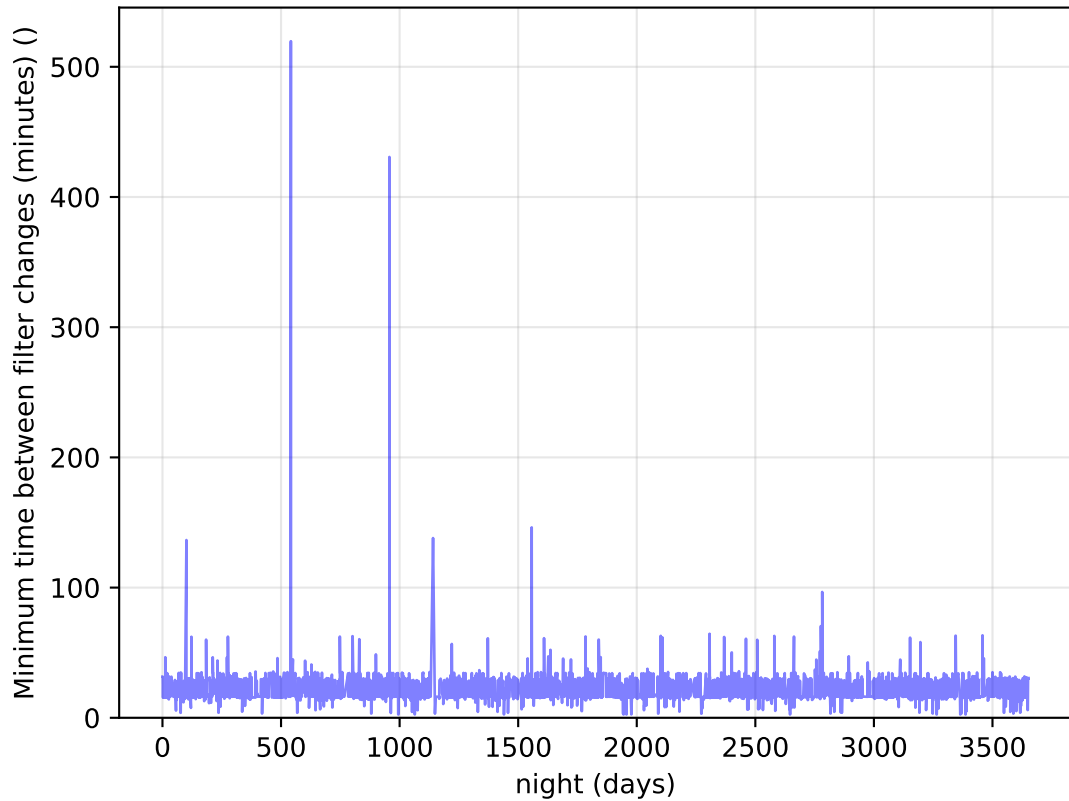
ddf_loaded_fl8_v3.4_10yrs Per Night: Minimum time between filter changes (minutes)
