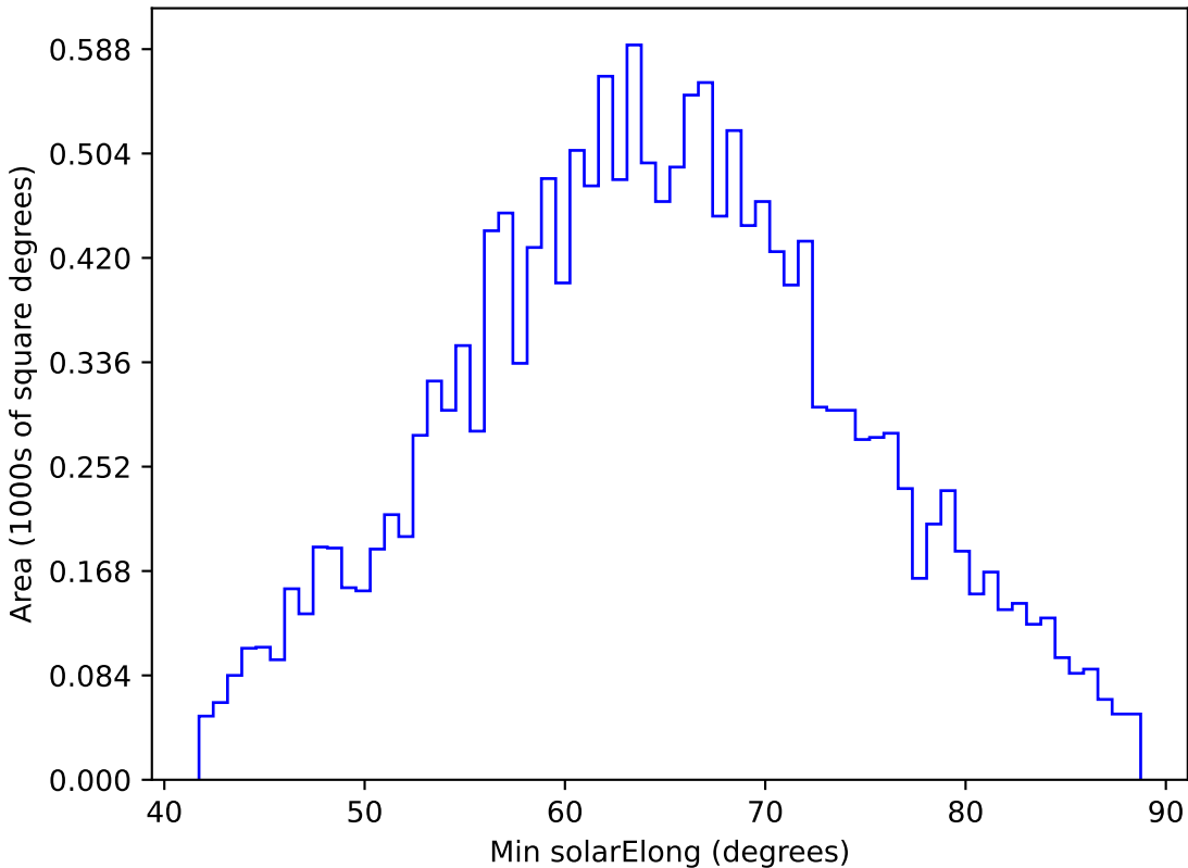
ddf_loaded_fl8_v3.4_10yrs WFD y band: Min solarElong
