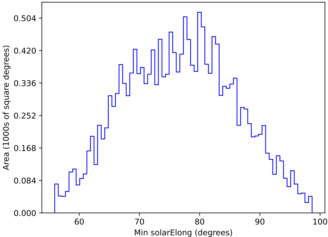
ddf_loaded_fl8_v3.4_10yrs WFD u band: Min solarElong
