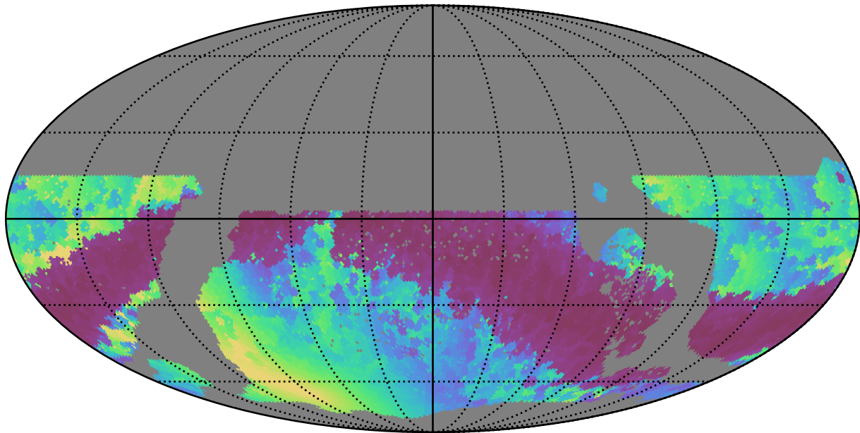
ddf_loaded_fl8_v3.4_10yrs WFD r band: Min solarElong
