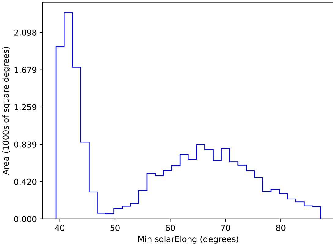
ddf_loaded_fl8_v3.4_10yrs WFD r band: Min solarElong
