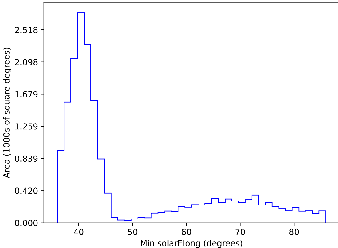
ddf_loaded_fl8_v3.4_10yrs WFD i band: Min solarElong
