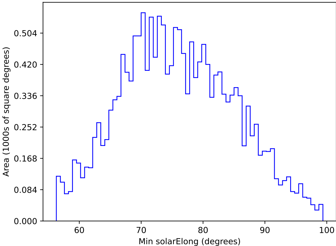
ddf_loaded_fl8_v3.4_10yrs WFD g band: Min solarElong
