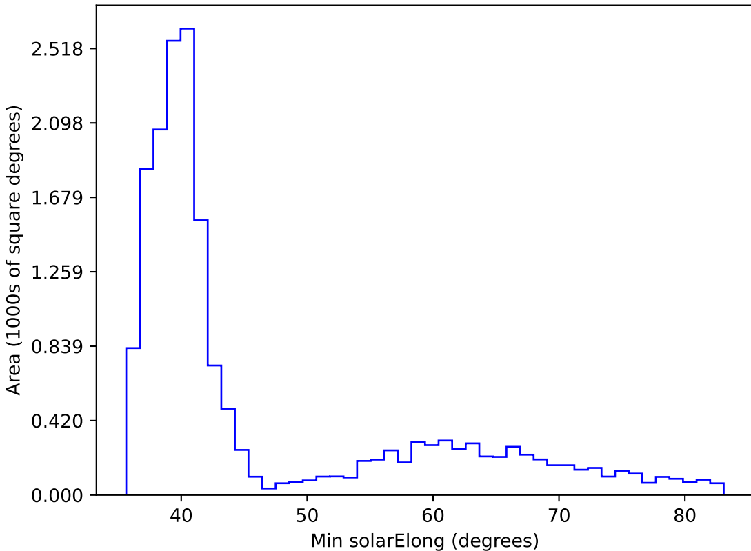
ddf_loaded_fl8_v3.4_10yrs WFD all bands: Min solarElong
