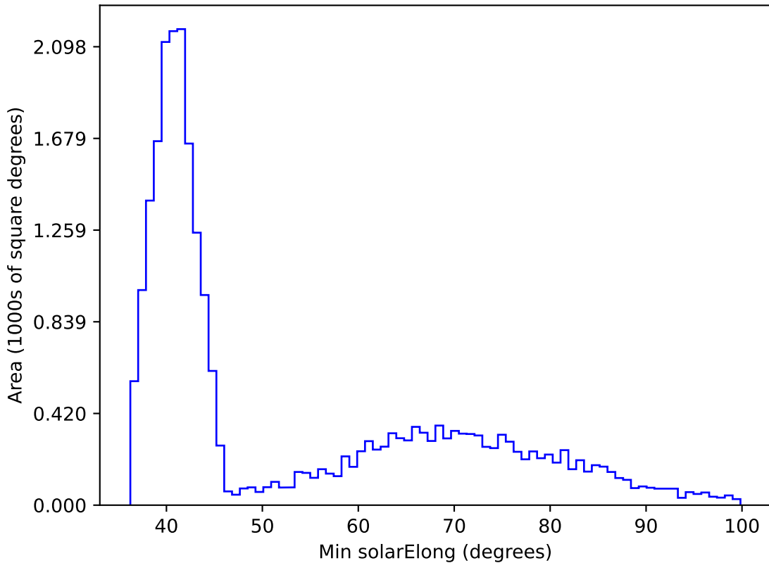
ddf_loaded_fl8_v3.4_10yrs All sky z band: Min solarElong
