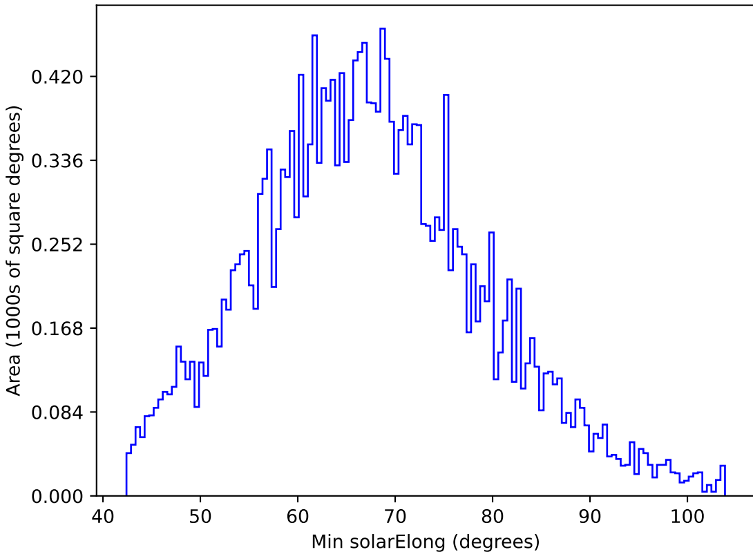
ddf_loaded_fl8_v3.4_10yrs All sky y band: Min solarElong
