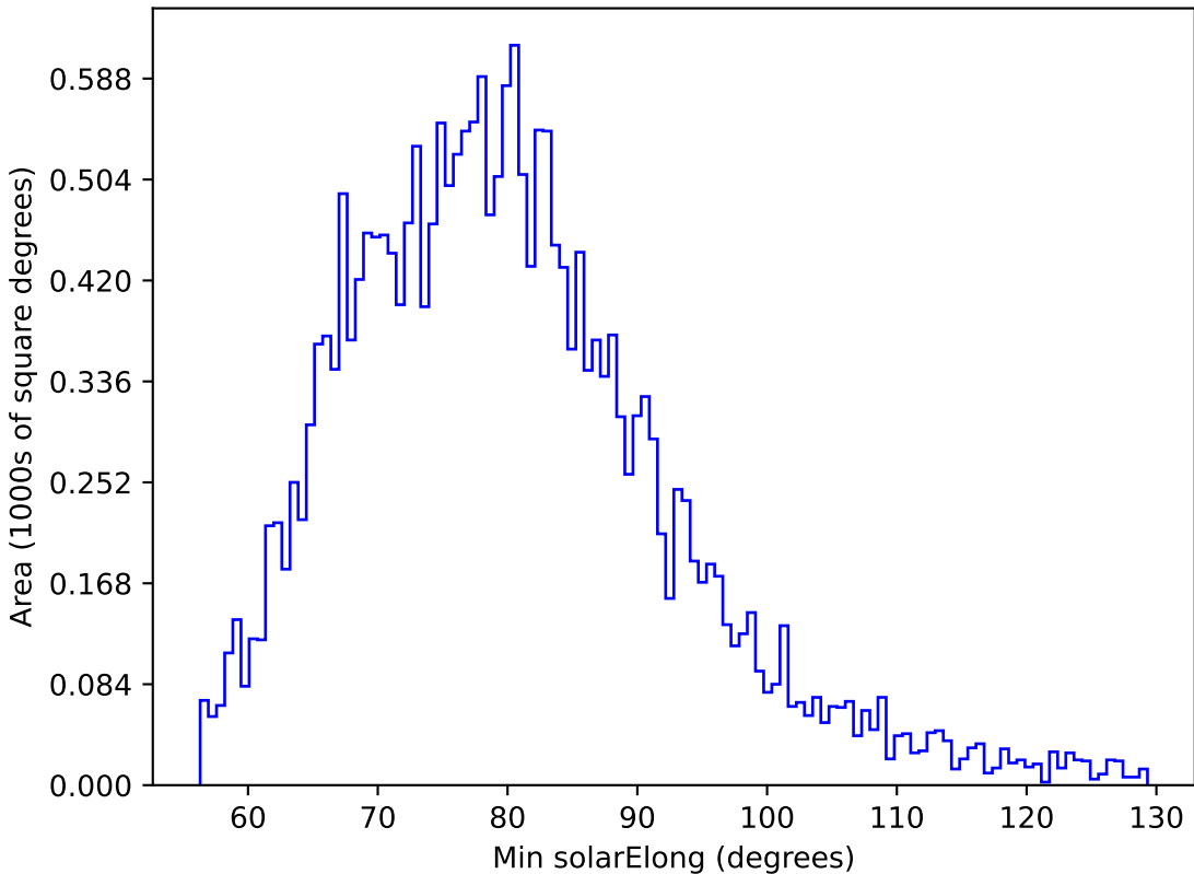
ddf_loaded_fl8_v3.4_10yrs All sky u band: Min solarElong
