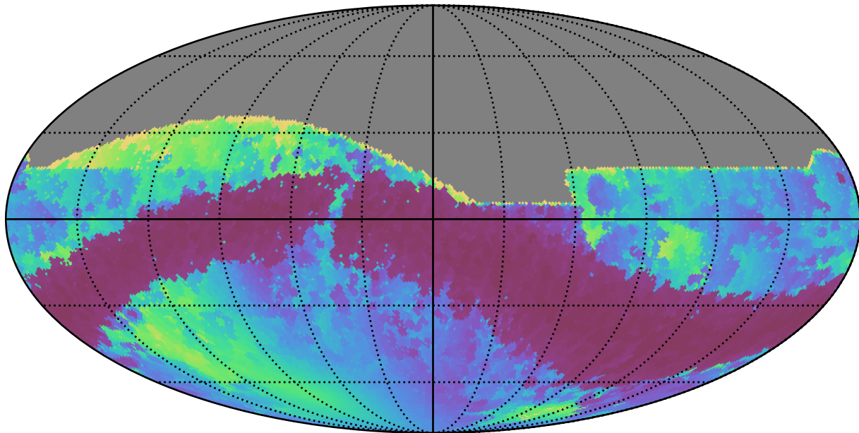
ddf_loaded_fl8_v3.4_10yrs All sky r band: Min solarElong
