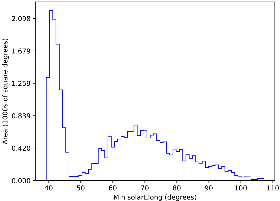
ddf_loaded_fl8_v3.4_10yrs All sky r band: Min solarElong
