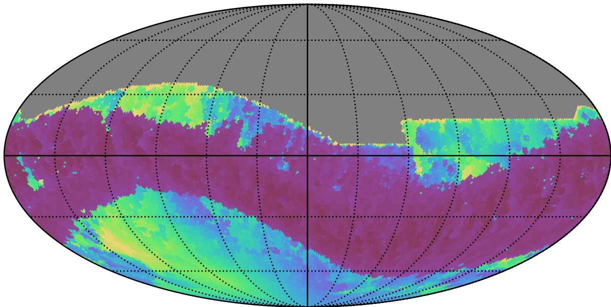
ddf_loaded_fl8_v3.4_10yrs All sky i band: Min solarElong
