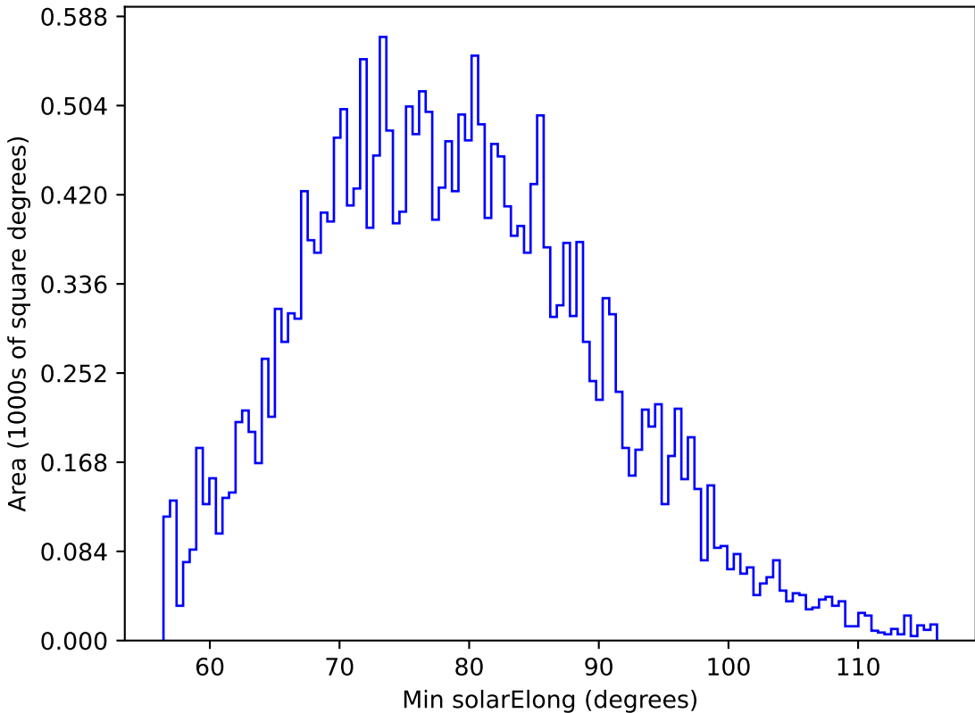
ddf_loaded_fl8_v3.4_10yrs All sky g band: Min solarElong
