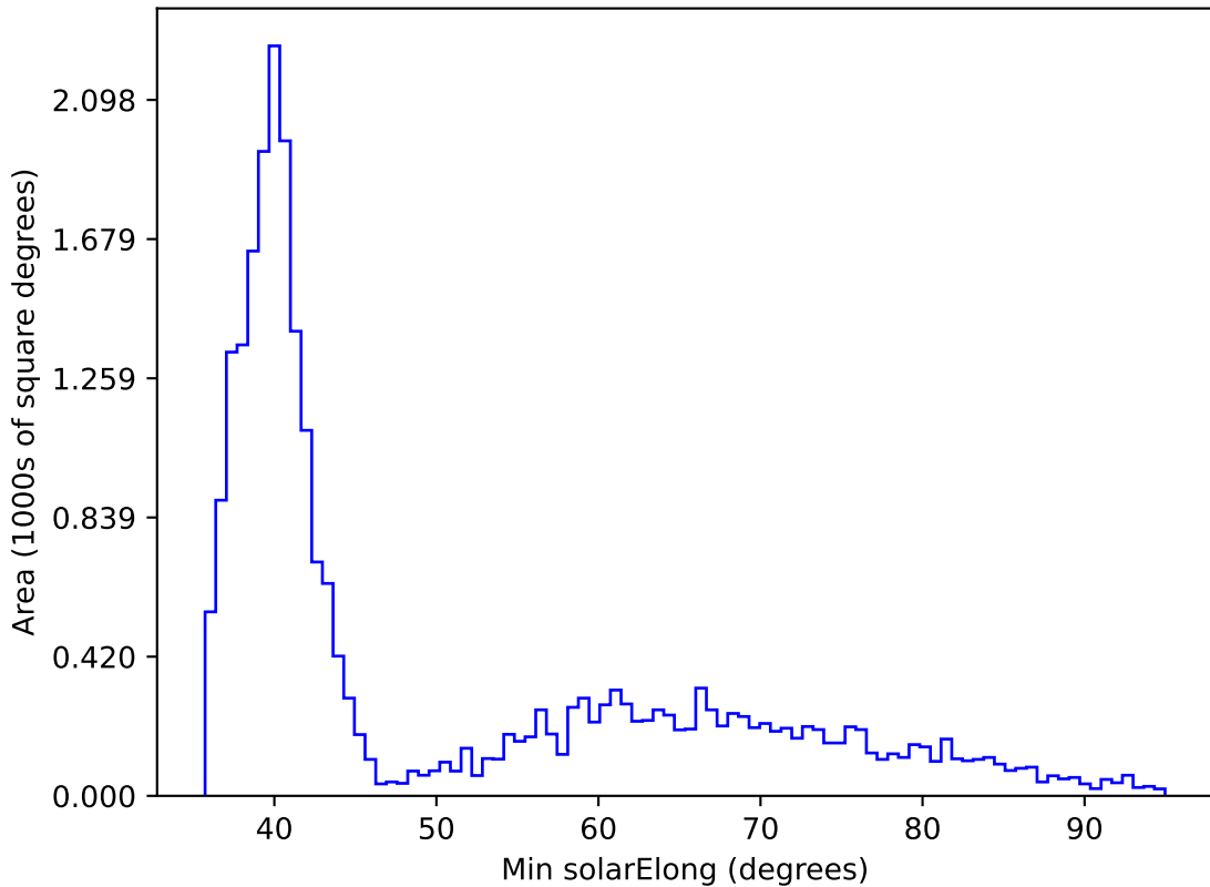
ddf_loaded_fl8_v3.4_10yrs All sky all bands: Min solarElong
