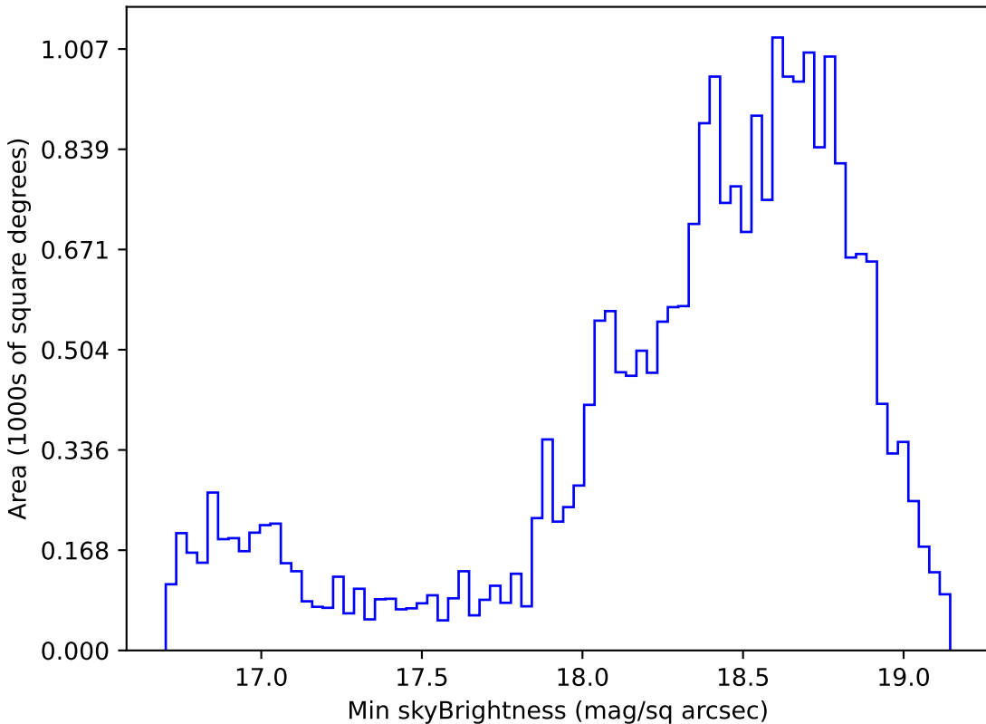
ddf_loaded_fl8_v3.4_10yrs Yr 1 z band: Min skyBrightness
