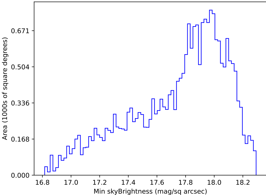
ddf_loaded_fl8_v3.4_10yrs Yr 1 y band: Min skyBrightness
