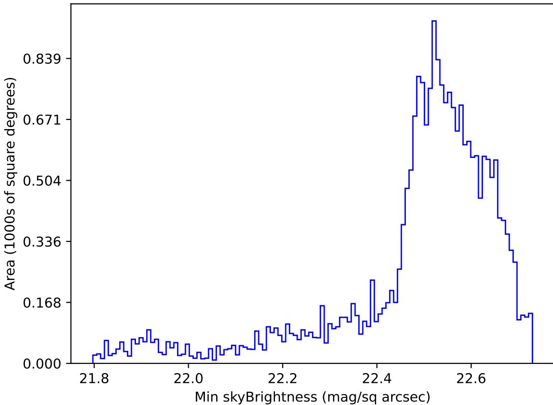
ddf_loaded_fl8_v3.4_10yrs Yr 1 u band: Min skyBrightness
