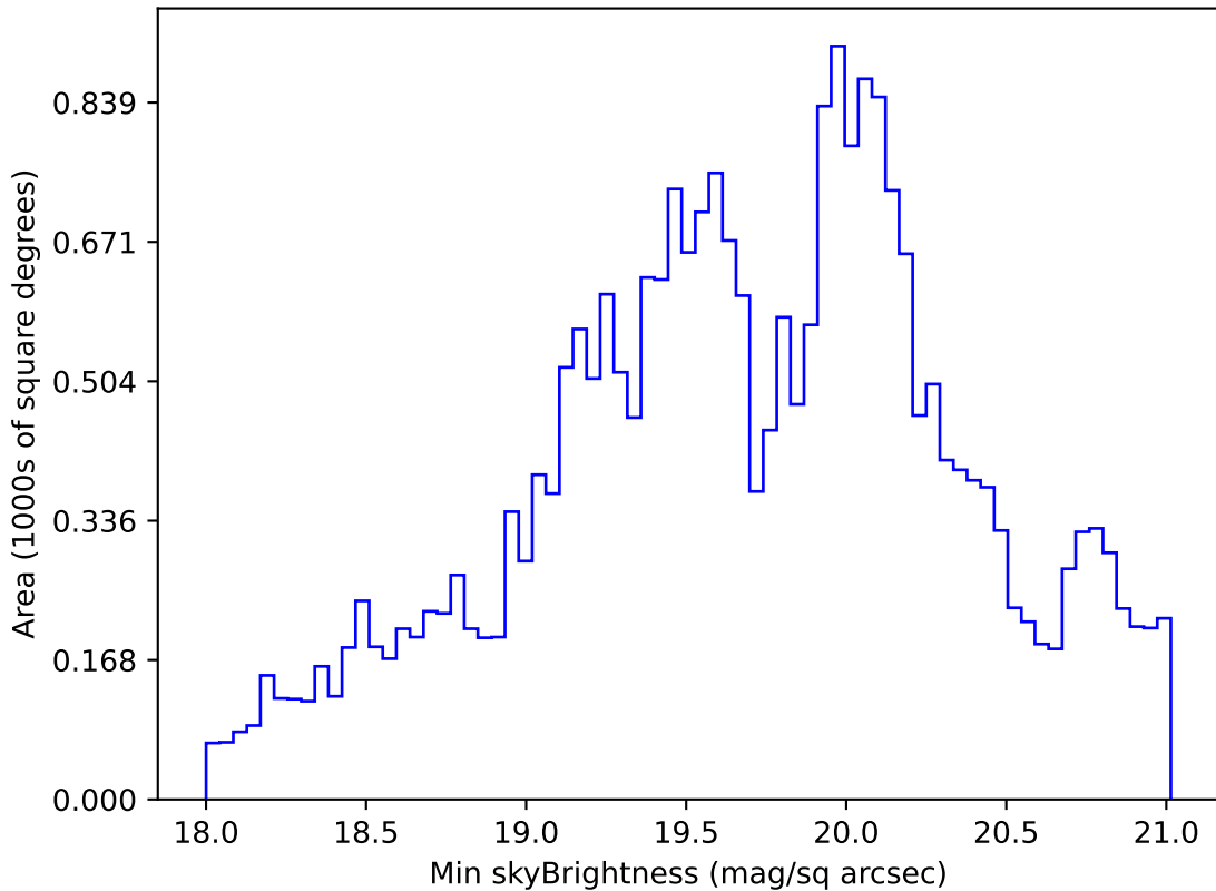
ddf_loaded_fl8_v3.4_10yrs Yr 1 r band: Min skyBrightness
