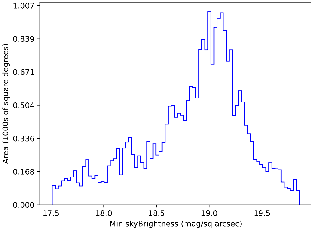
ddf_loaded_fl8_v3.4_10yrs Yr 1 i band: Min skyBrightness
