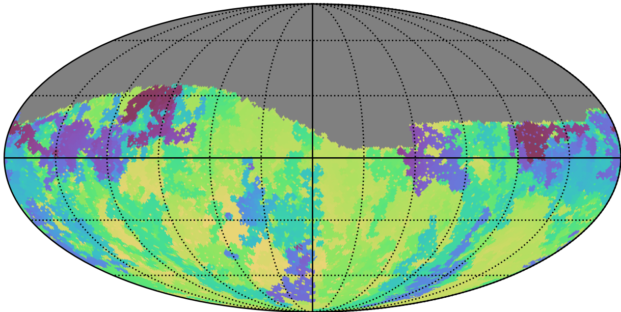
ddf_loaded_fl8_v3.4_10yrs Yr 1 g band: Min skyBrightness
