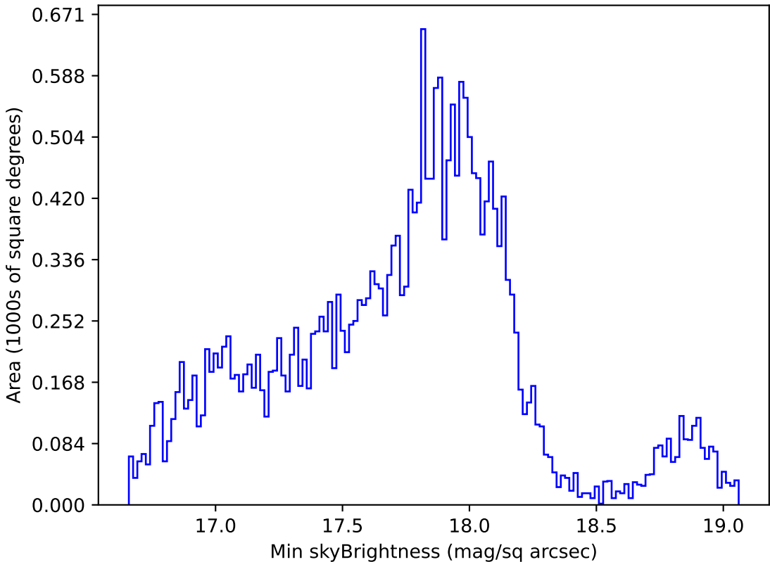
ddf_loaded_fl8_v3.4_10yrs Yr 1 all bands: Min skyBrightness
