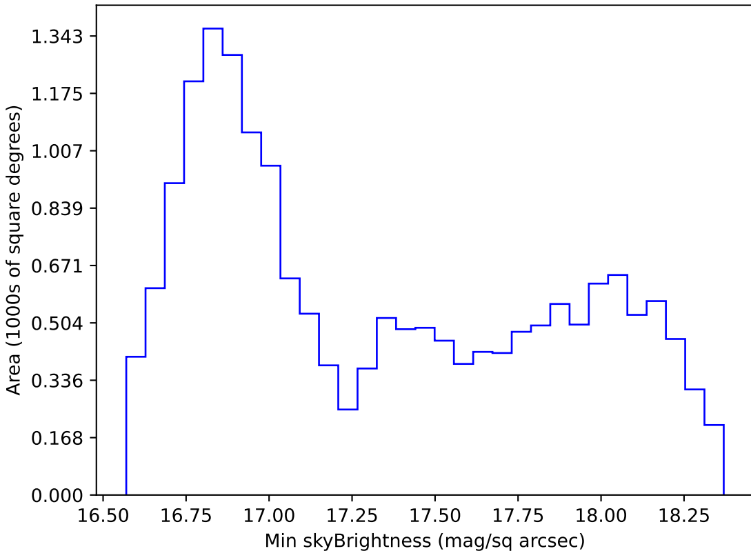
ddf_loaded_fl8_v3.4_10yrs WFD z band: Min skyBrightness
