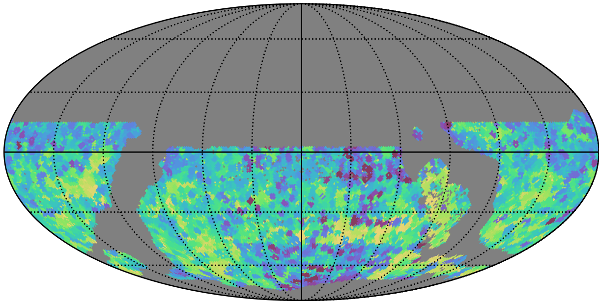
ddf_loaded_fl8_v3.4_10yrs WFD y band: Min skyBrightness
