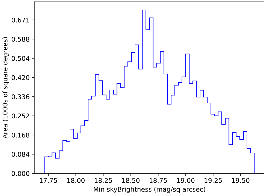
ddf_loaded_fl8_v3.4_10yrs WFD r band: Min skyBrightness
