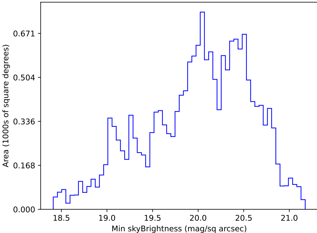
ddf_loaded_fl8_v3.4_10yrs WFD g band: Min skyBrightness
