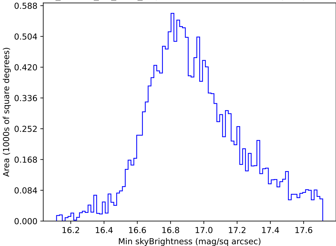
ddf_loaded_fl8_v3.4_10yrs WFD all bands: Min skyBrightness
