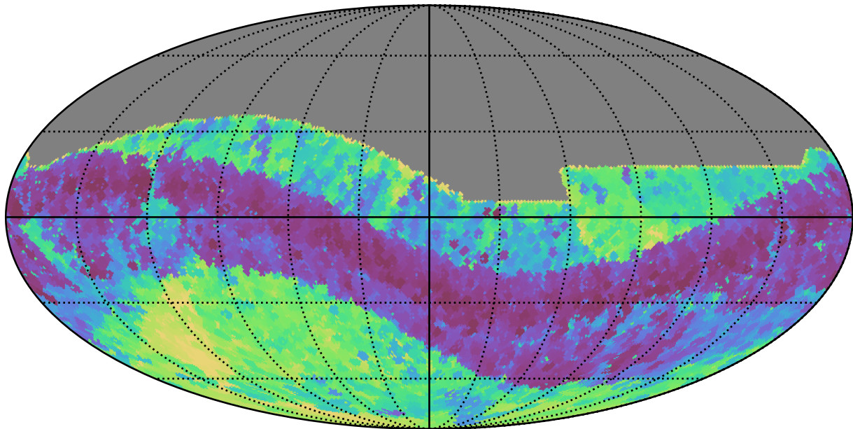
ddf_loaded_fl8_v3.4_10yrs All sky z band: Min skyBrightness
