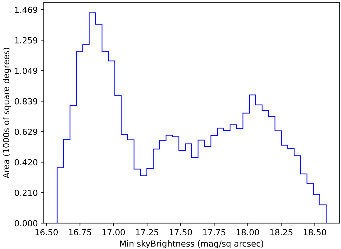
ddf_loaded_fl8_v3.4_10yrs All sky z band: Min skyBrightness
