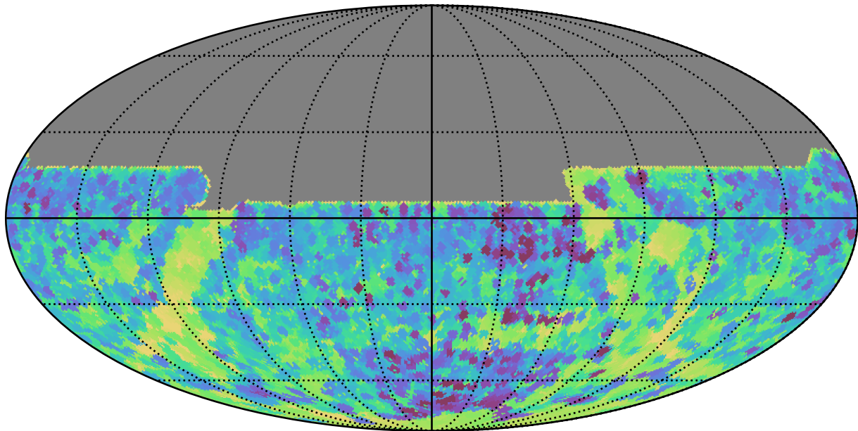
ddf_loaded_fl8_v3.4_10yrs All sky y band: Min skyBrightness
