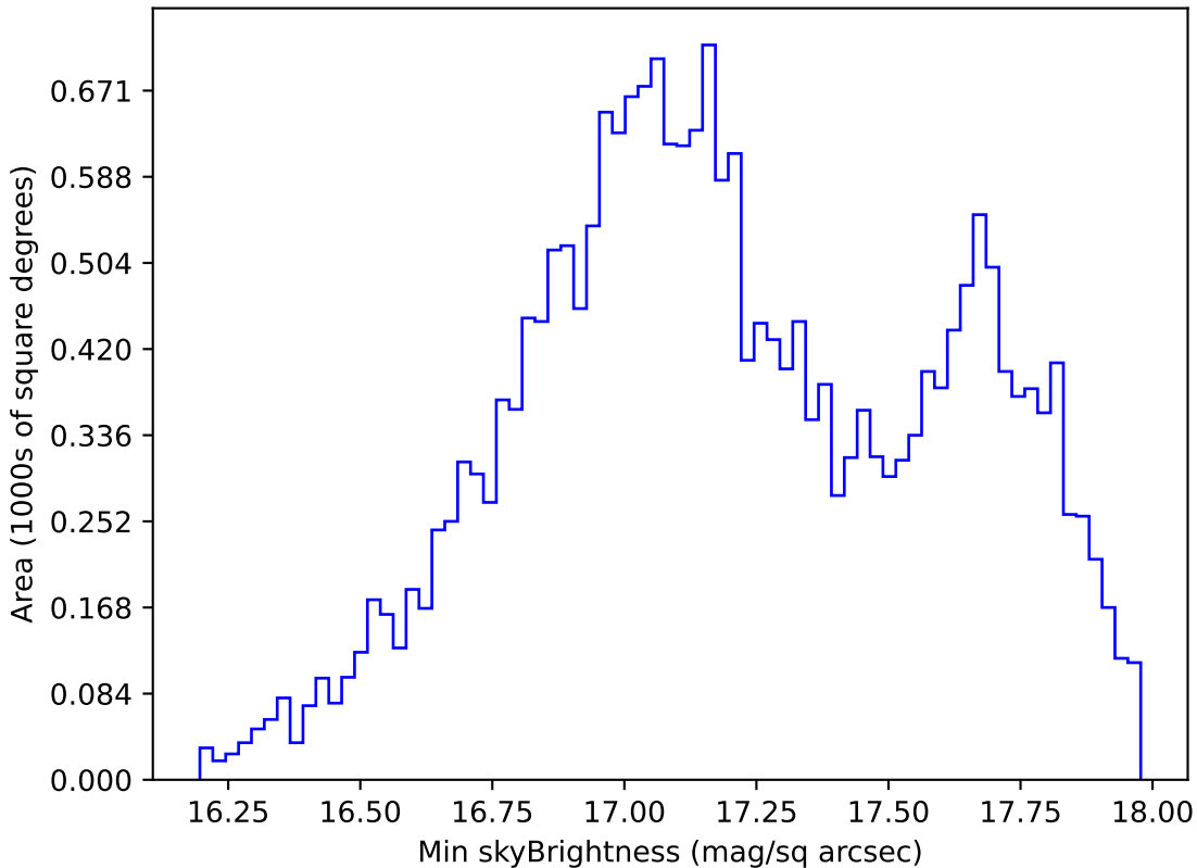
ddf_loaded_fl8_v3.4_10yrs All sky y band: Min skyBrightness
