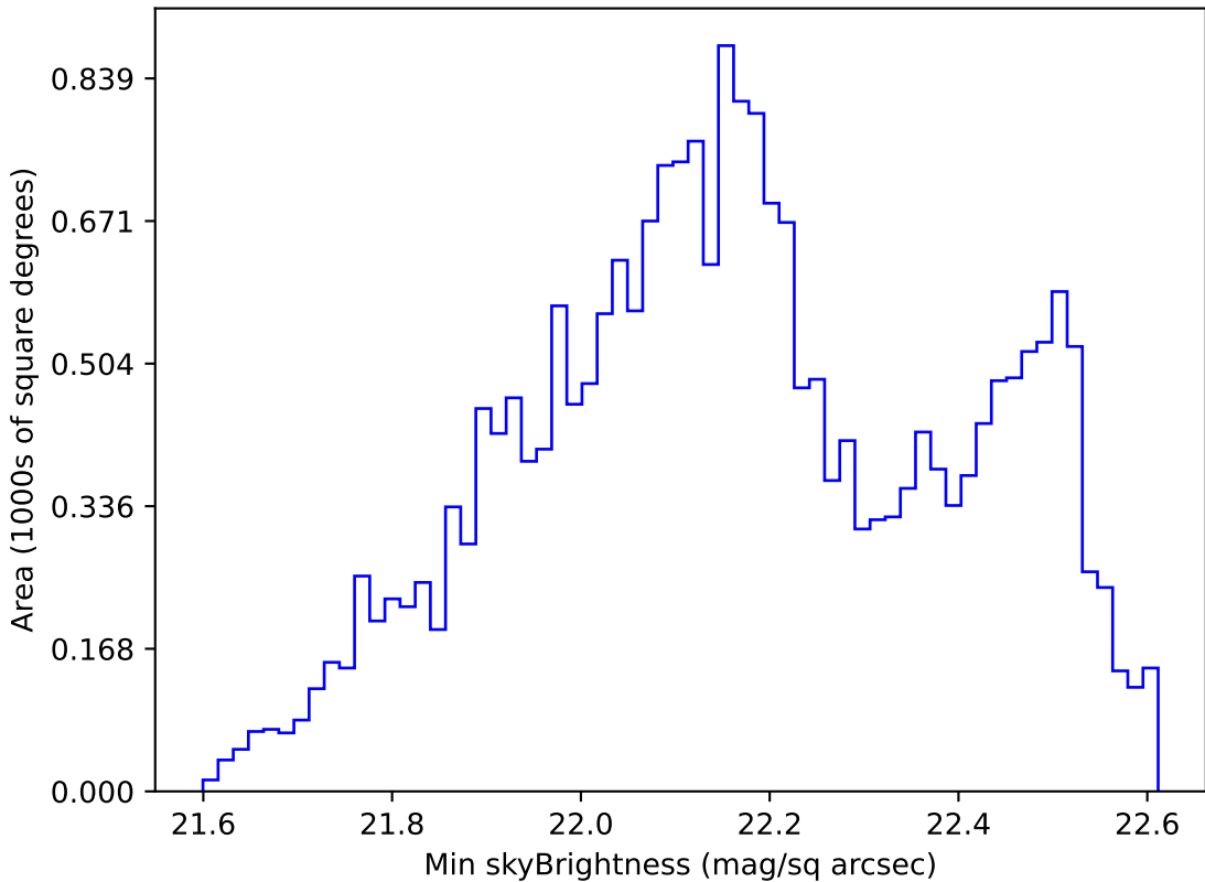
ddf_loaded_fl8_v3.4_10yrs All sky u band: Min skyBrightness
