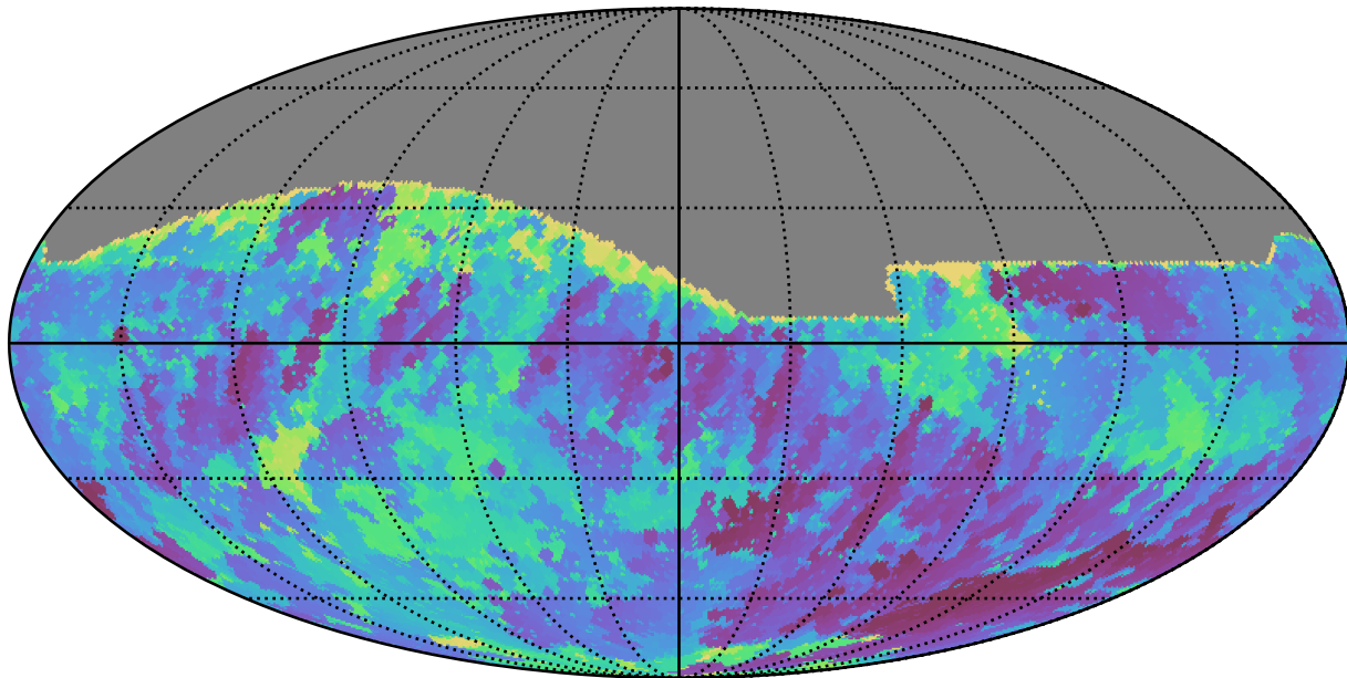
ddf_loaded_fl8_v3.4_10yrs All sky r band: Min skyBrightness
