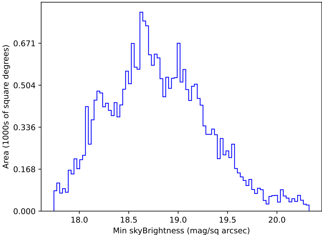
ddf_loaded_fl8_v3.4_10yrs All sky r band: Min skyBrightness
