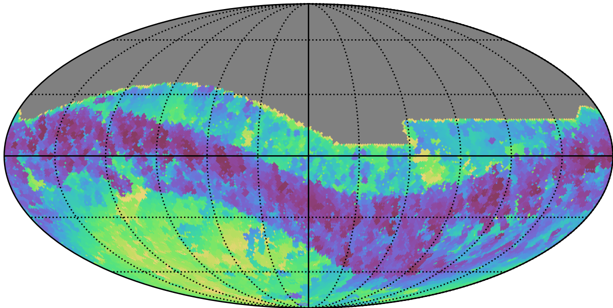
ddf_loaded_fl8_v3.4_10yrs All sky i band: Min skyBrightness
