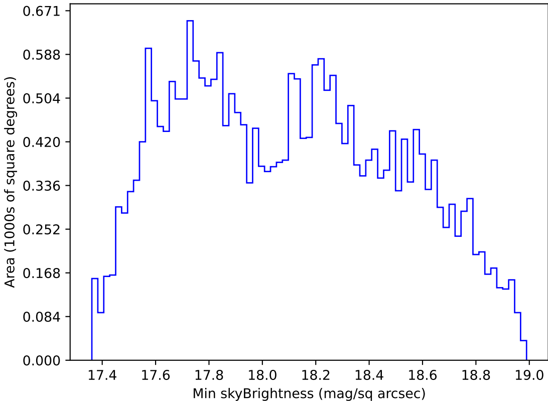
ddf_loaded_fl8_v3.4_10yrs All sky i band: Min skyBrightness
